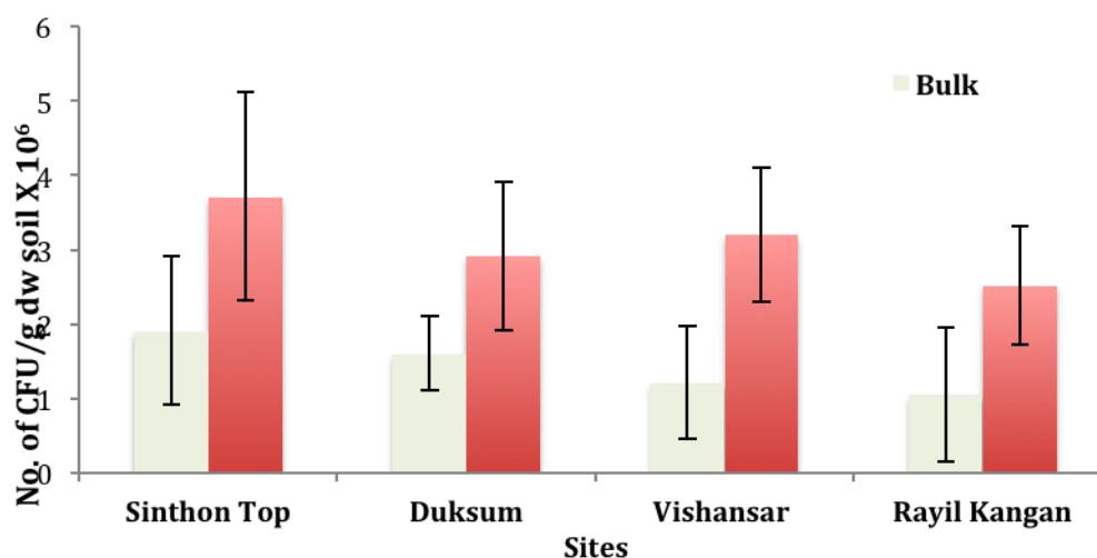
Fig 2. Enumeration of bacterial diversity from rhizosphere and bulk soil from the roots of A. benthamii from four sites
