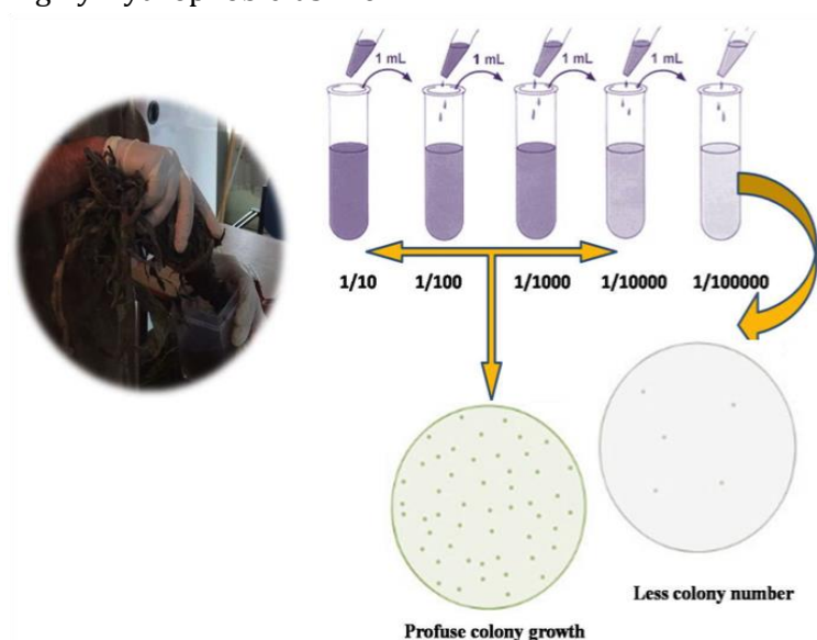
Fig1. Diagrammatic representation of developed protocol of isolation and enumeration of rhizobacteria.
